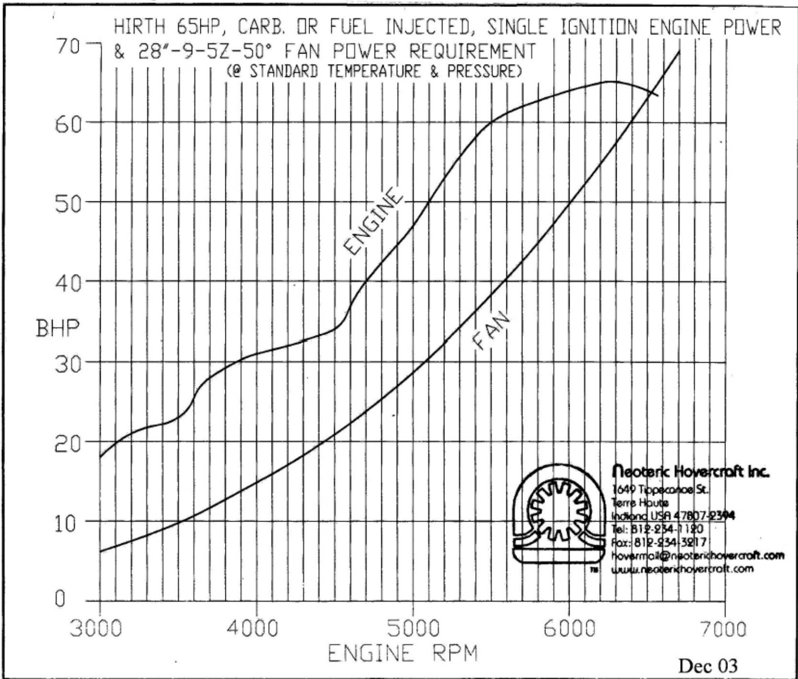
Hirth 65HP Engine Fan Curve
