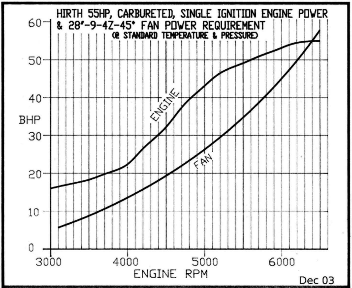
HIRTH 55 HP ENGINE FAN CURVE
