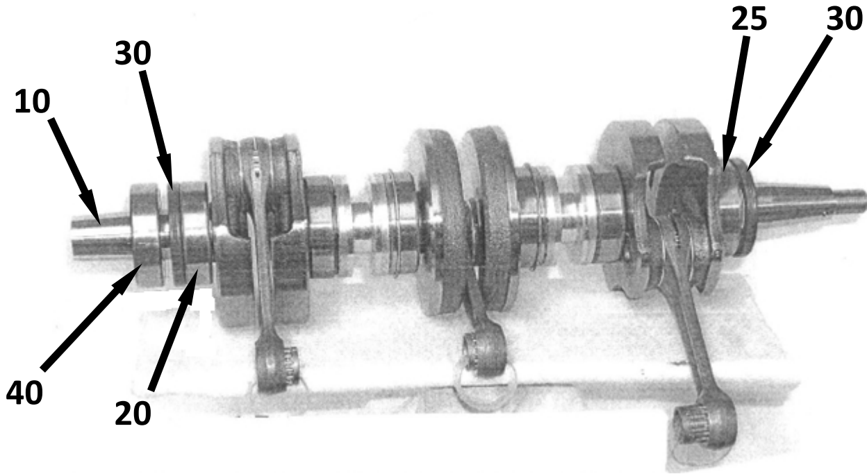
complete crankshaft contains Pos. 10-40
